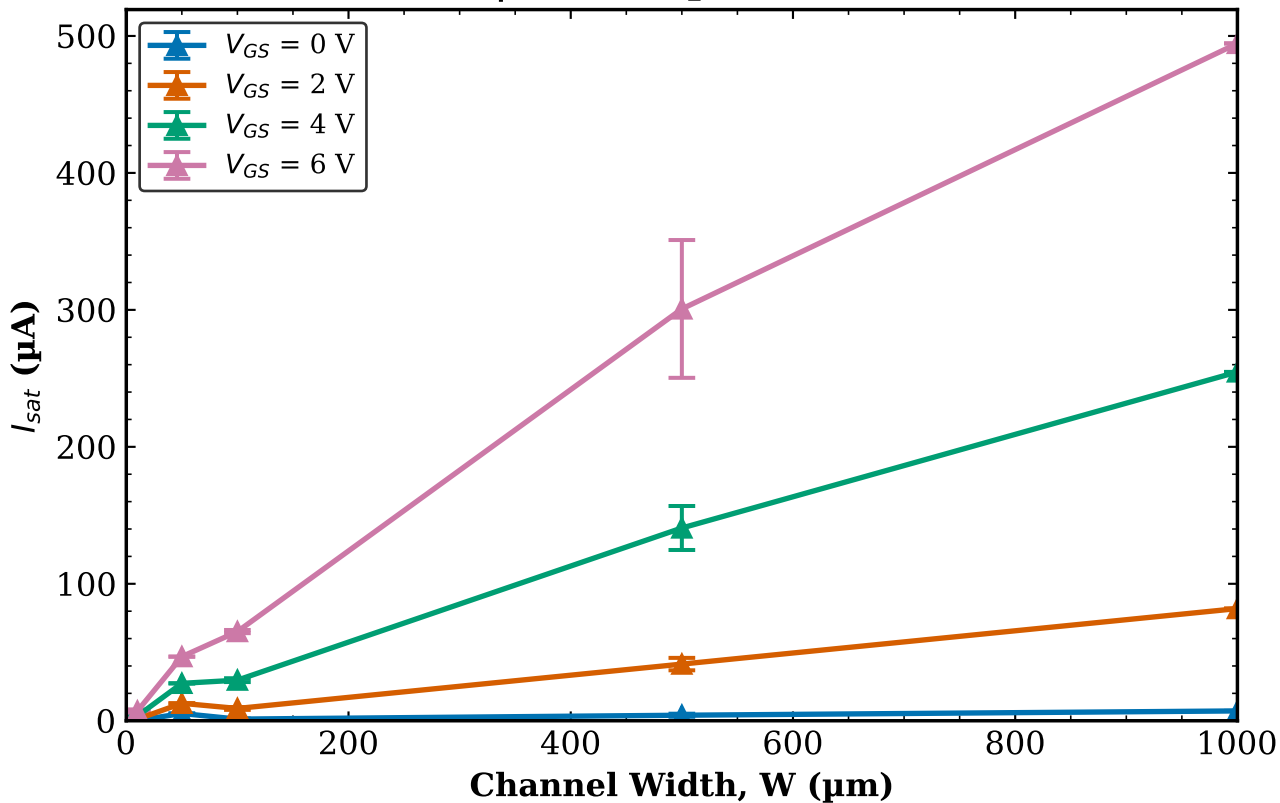
TFT1 Combined (Tr. 1 & 2) I_{sat} vs W | L = 20\text{ }\mu\text{m} (mean \pm std)
